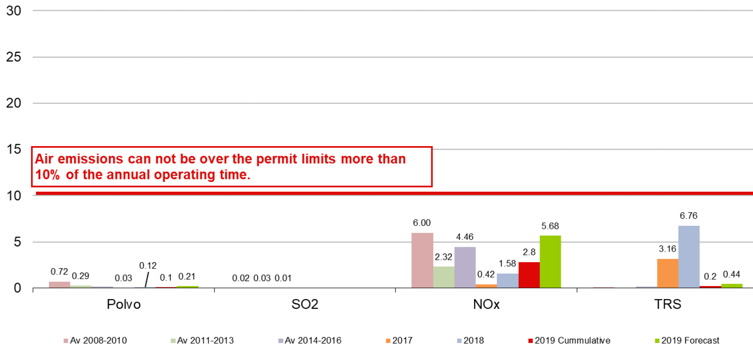
Lime Kiln- % of time over permit limit
