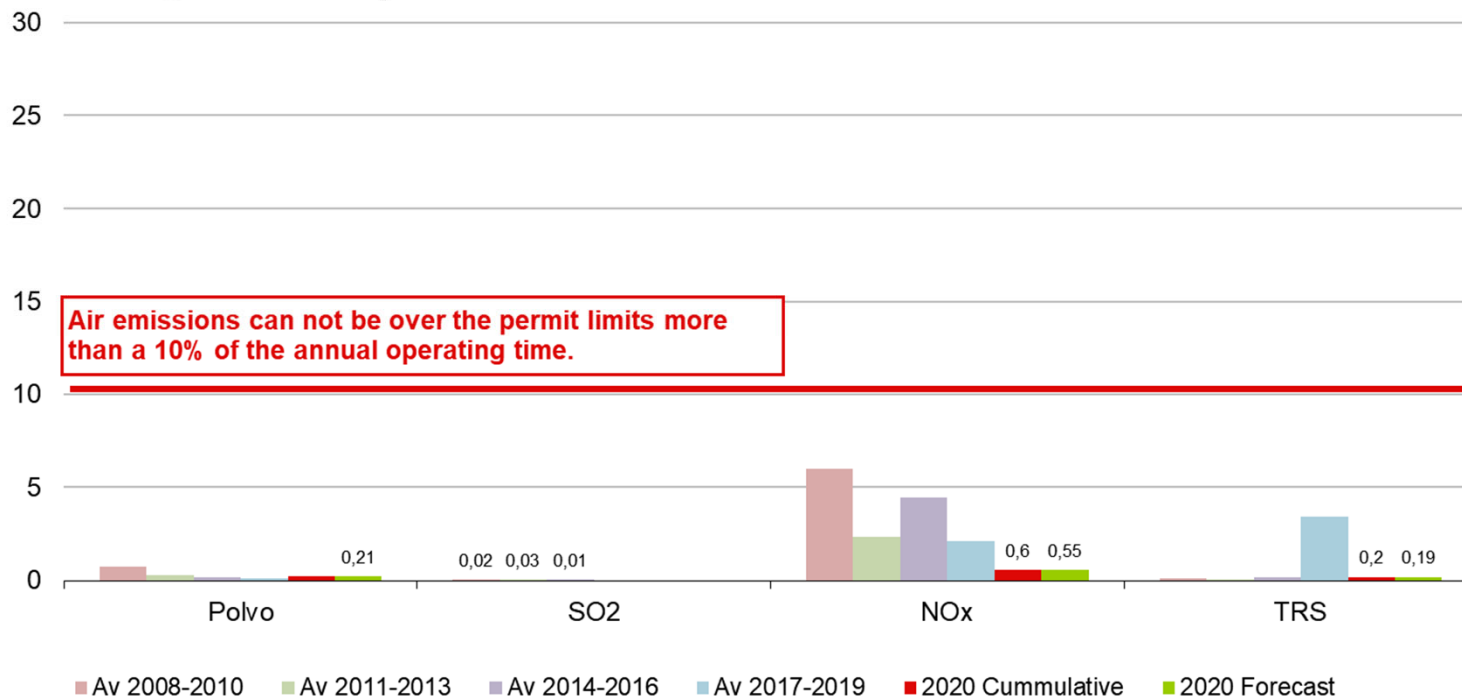
Lime kiln - % of time over permit limit
