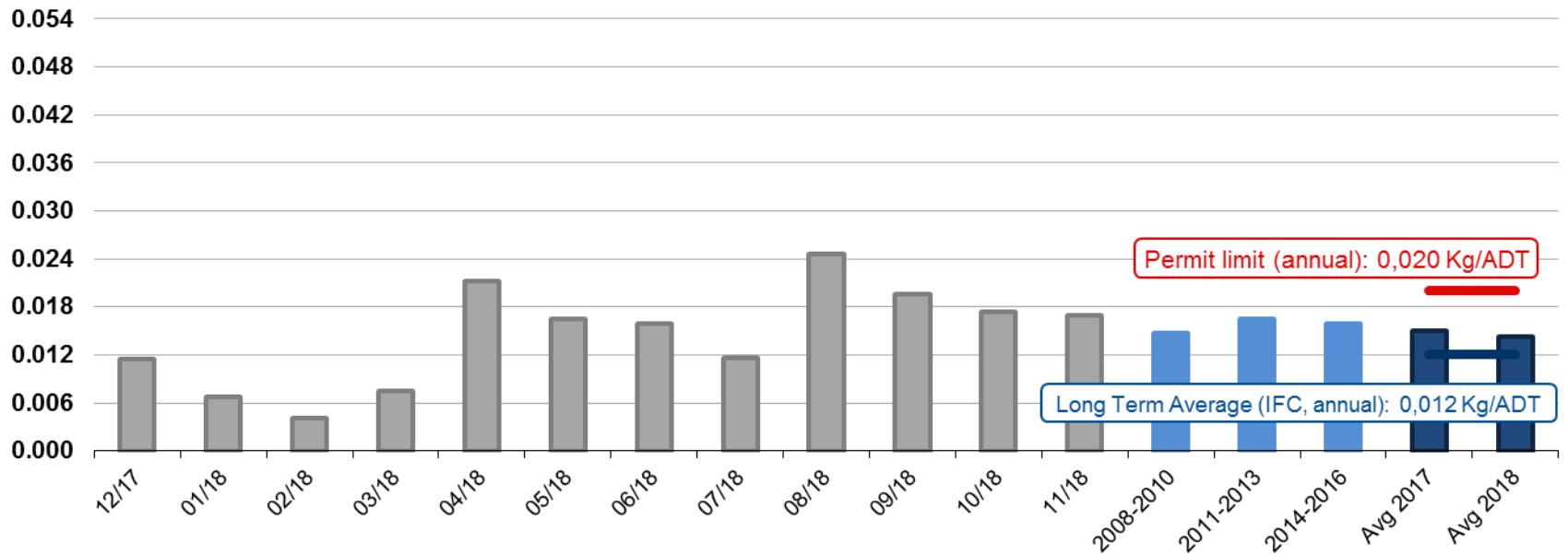
P Total - Kg/ADT
