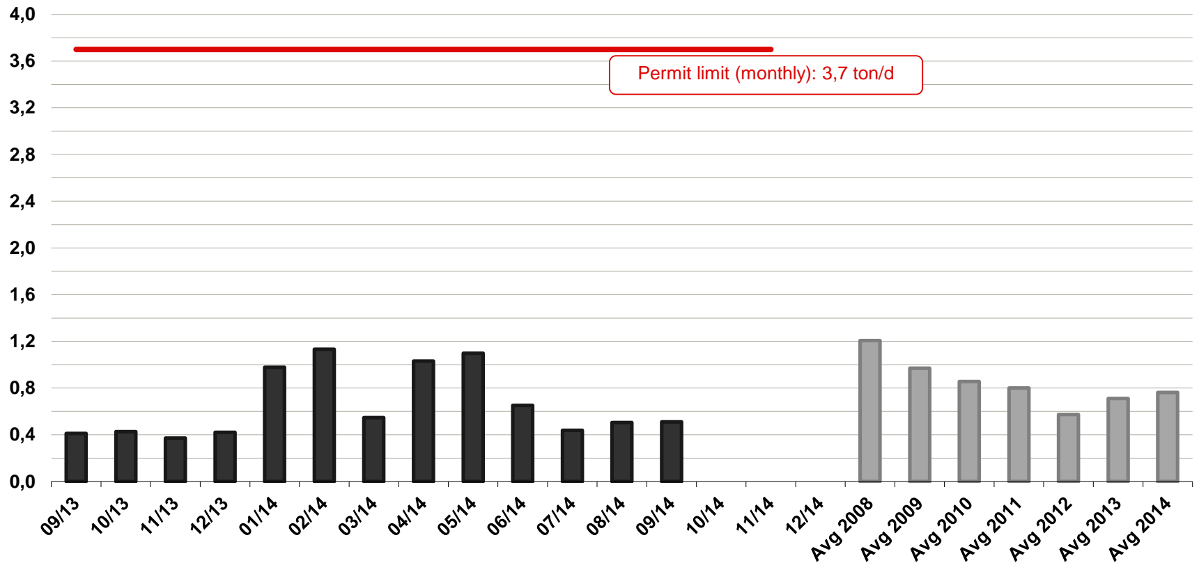
TSS - ton/d
